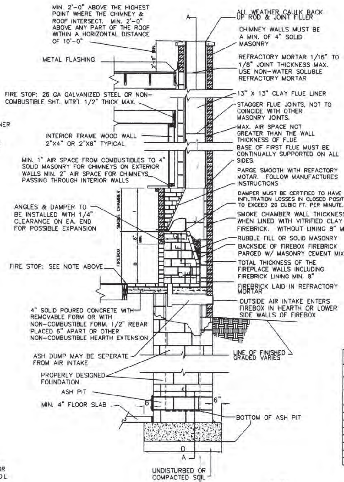
SECTION B-B
